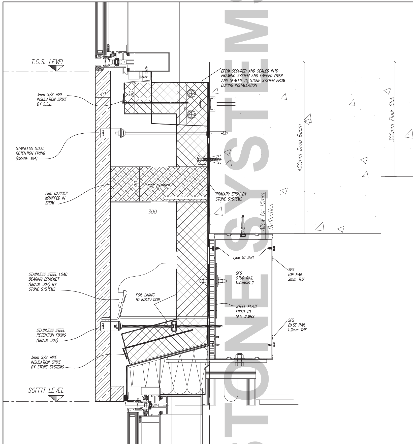
TYPICAL SOFFIT & FLUSH CILL DETAIL SCALE: 1:5
