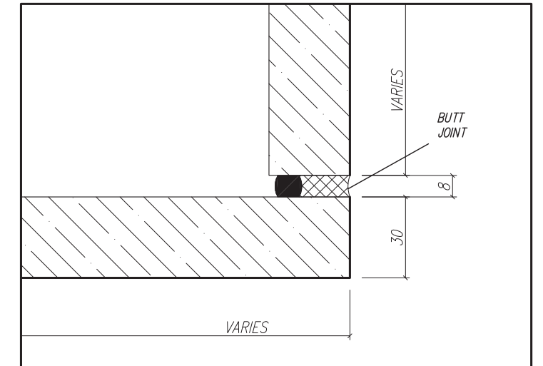
GLUED & PINNED BUTT JOINT SCALE: 1:2
