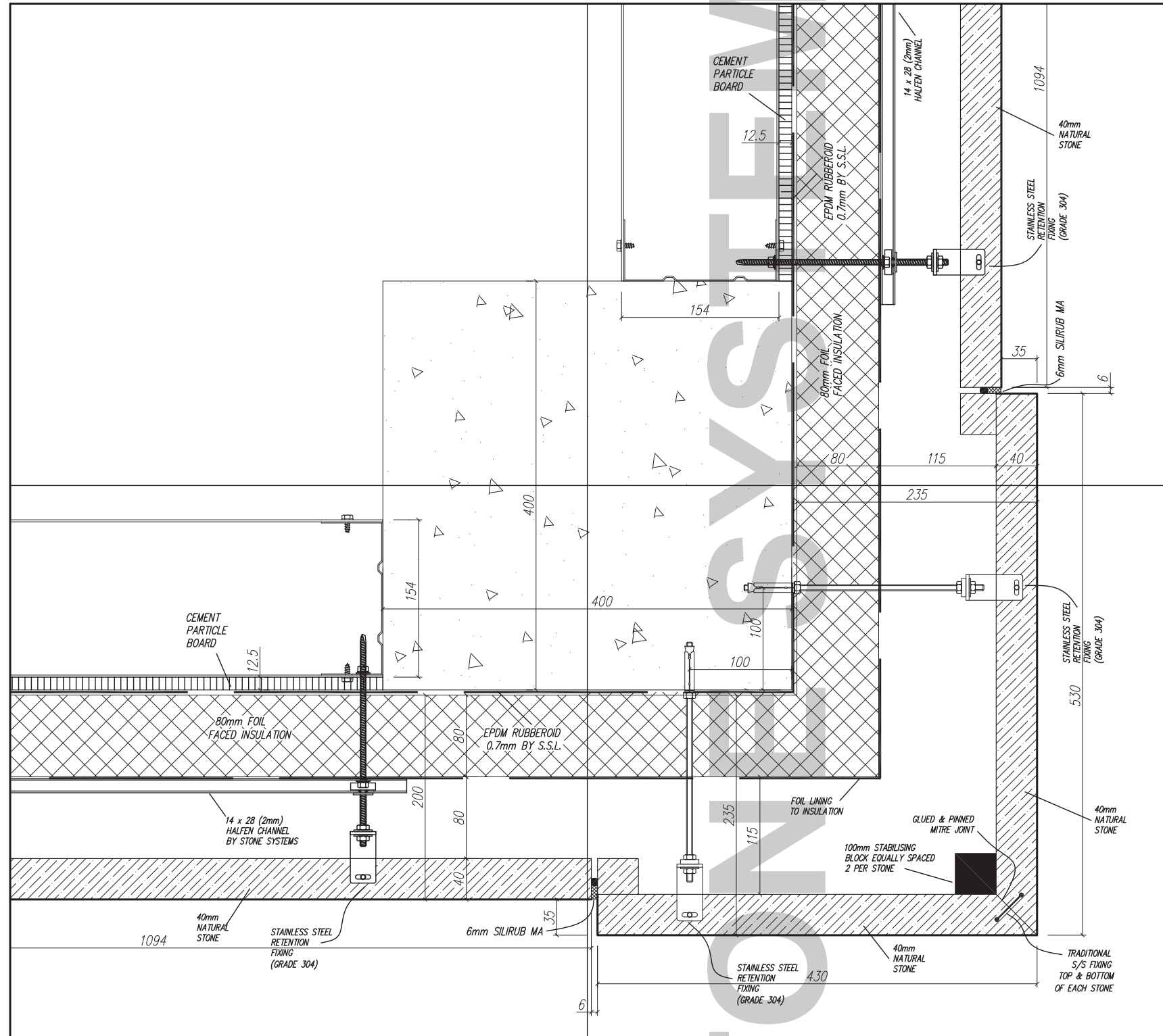
CORNER DETAIL: GLUED & PINNED MITRE JOINT SCALE: 1:5
