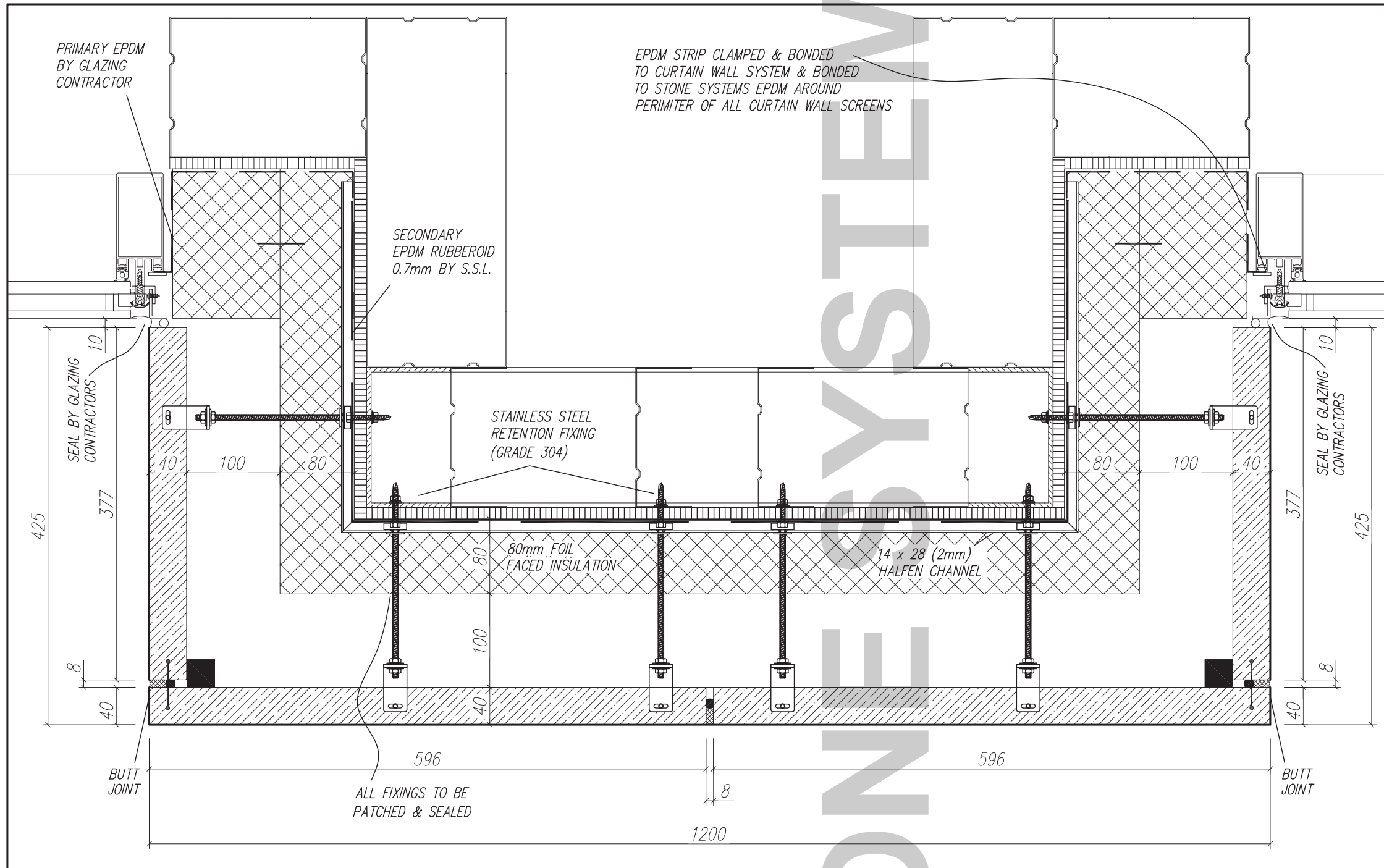
COLUMN DETAIL WITH SFS FIXING SYSTEM: SCALE: 1:5
