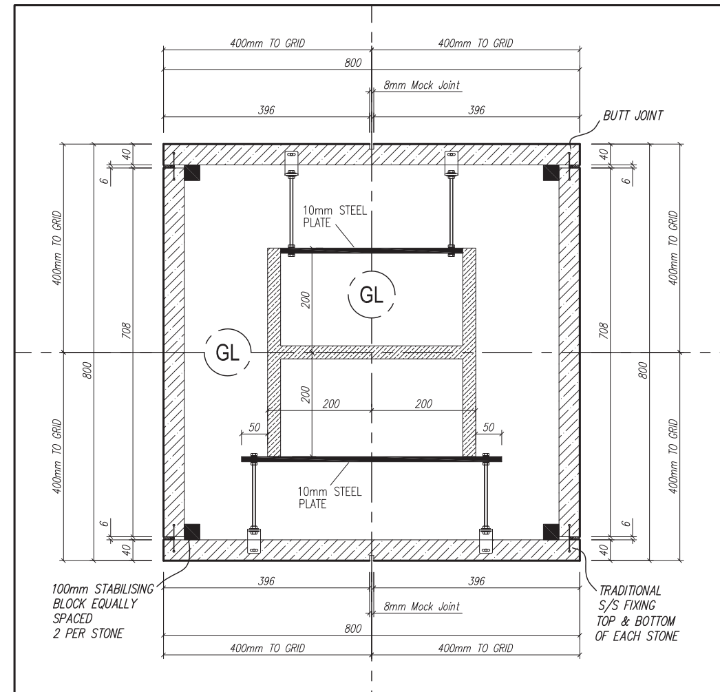
STEEL SUB COLUMN FRAME: ALTERNATIVE SCALE: 1:10
