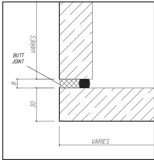
BUTT JOINT DETAIL: SCALE: 1:2
