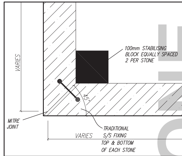
CLOSED MITRE JOINT DETAIL: SCALE: 1:2
