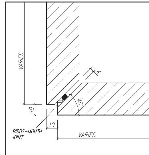
BIRDS-MOUTH DETAIL: SCALE: 1:2
