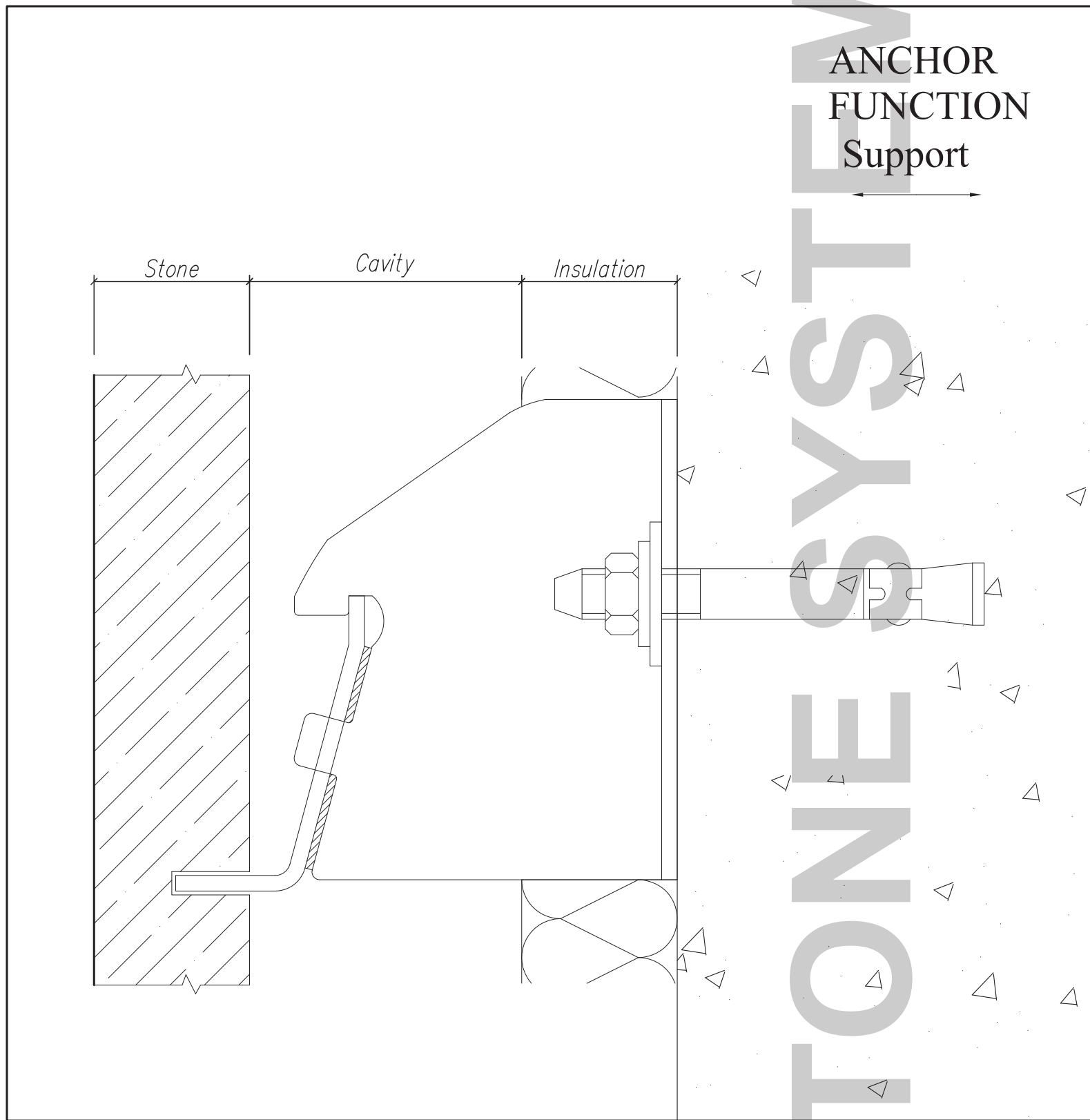
TYPICAL LOAD BEARING BRACKET DETAIL
