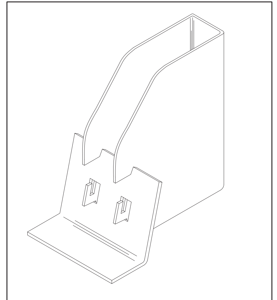
TYPICAL LOAD BEARING BRACKET ISO-VIEW
